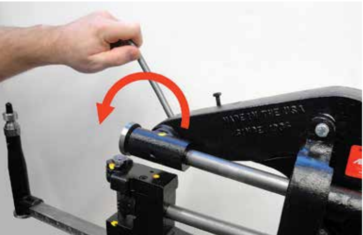
(Figure 4) Disengage the top cutting disc by rotating the cutting disc lever counter-clockwise.
